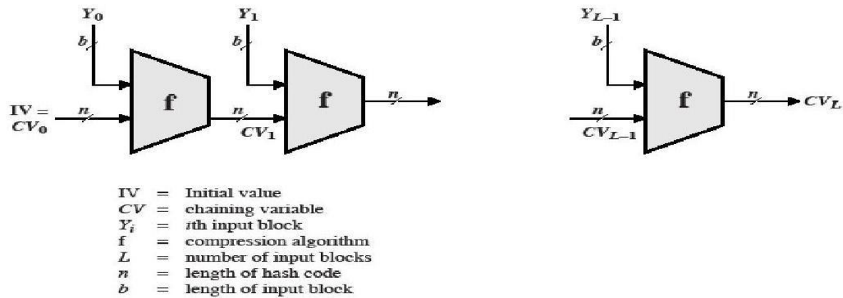
Fig.3.7.1: General Structure of Secure Hash Code
